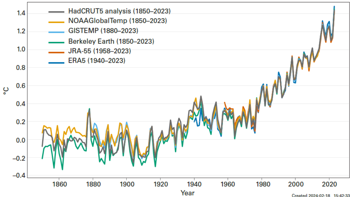
Figure 2. Annual global mean temperature anomalies (relative to 1850–1900)
